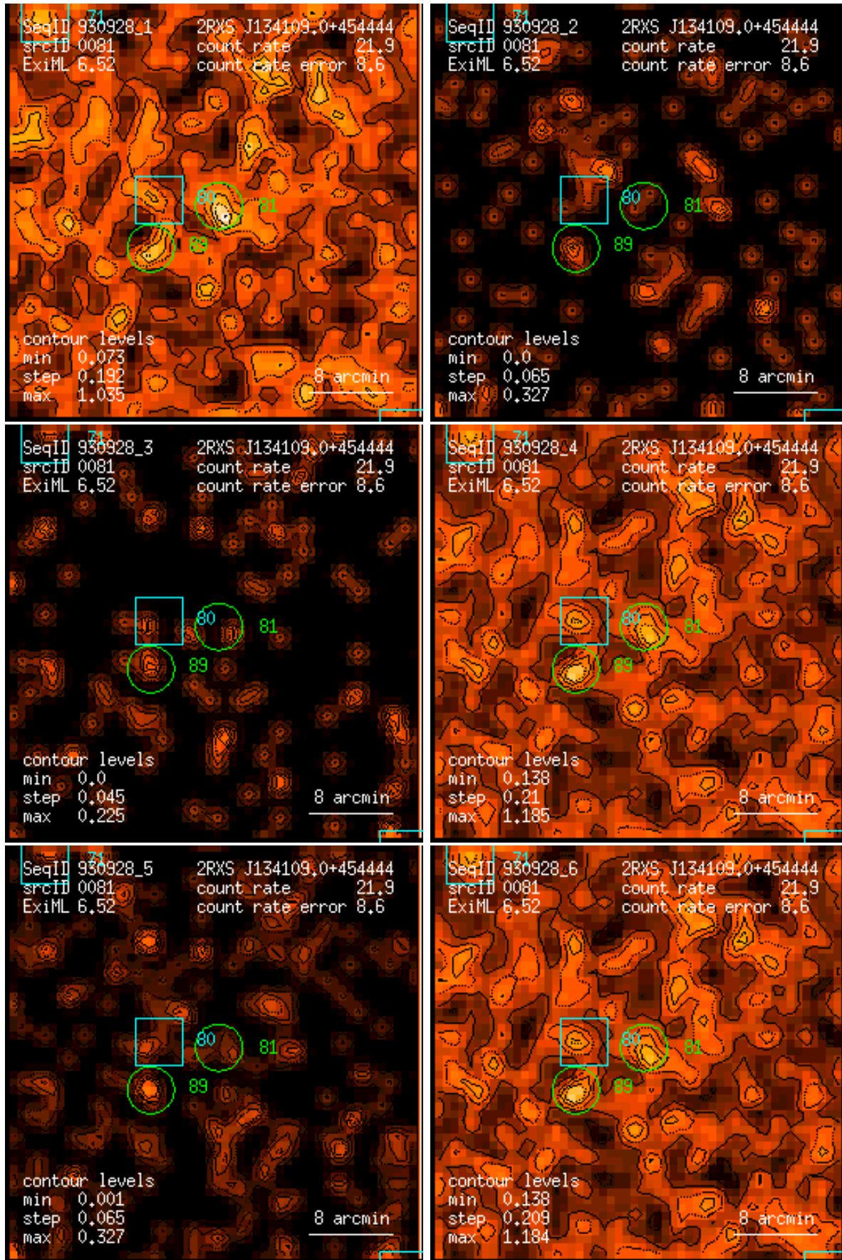
Figure 81: RASS 930928: detection 0081: band rate images, Gaussian filter: (1) PSPC channels 11 – 41, (2) 52 – 90, (3) 91 – 201, (4) 11 – 235, (5) 52 – 201, (6) 11 – 201. Broad band rates in counts/ks. Band rate contour levels in counts/ks/arcmin 2 .
