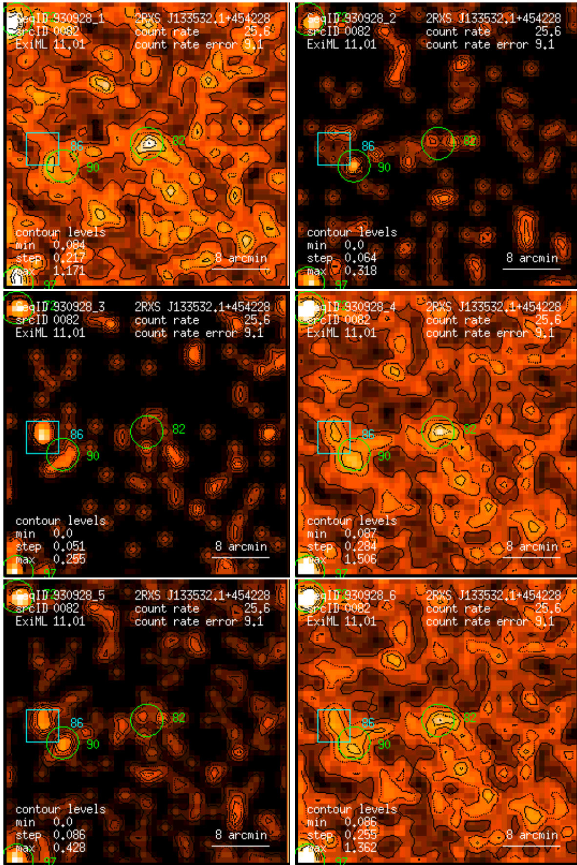
Figure 82: RASS 930928: detection 0082: band rate images, Gaussian filter: (1) PSPC channels 11 – 41, (2) 52 – 90, (3) 91 – 201, (4) 11 – 235, (5) 52 – 201, (6) 11 – 201. Broad band rates in counts/ks. Band rate contour levels in counts/ks/arcmin 2 .
