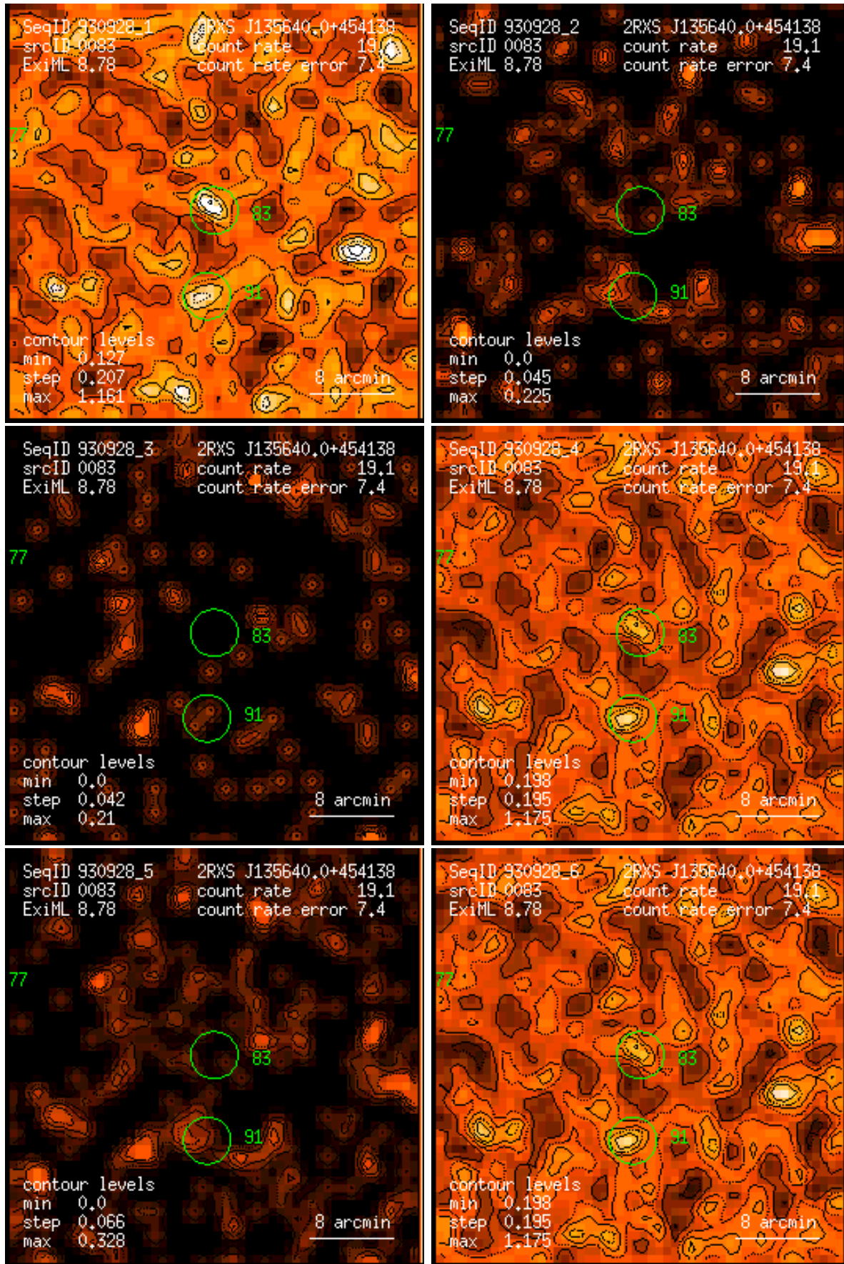
Figure 83: RASS 930928: detection 0083: band rate images, Gaussian filter: (1) PSPC channels 11 – 41, (2) 52 – 90, (3) 91 – 201, (4) 11 – 235, (5) 52 – 201, (6) 11 – 201. Broad band rates in counts/ks. Band rate contour levels in counts/ks/arcmin 2 .
