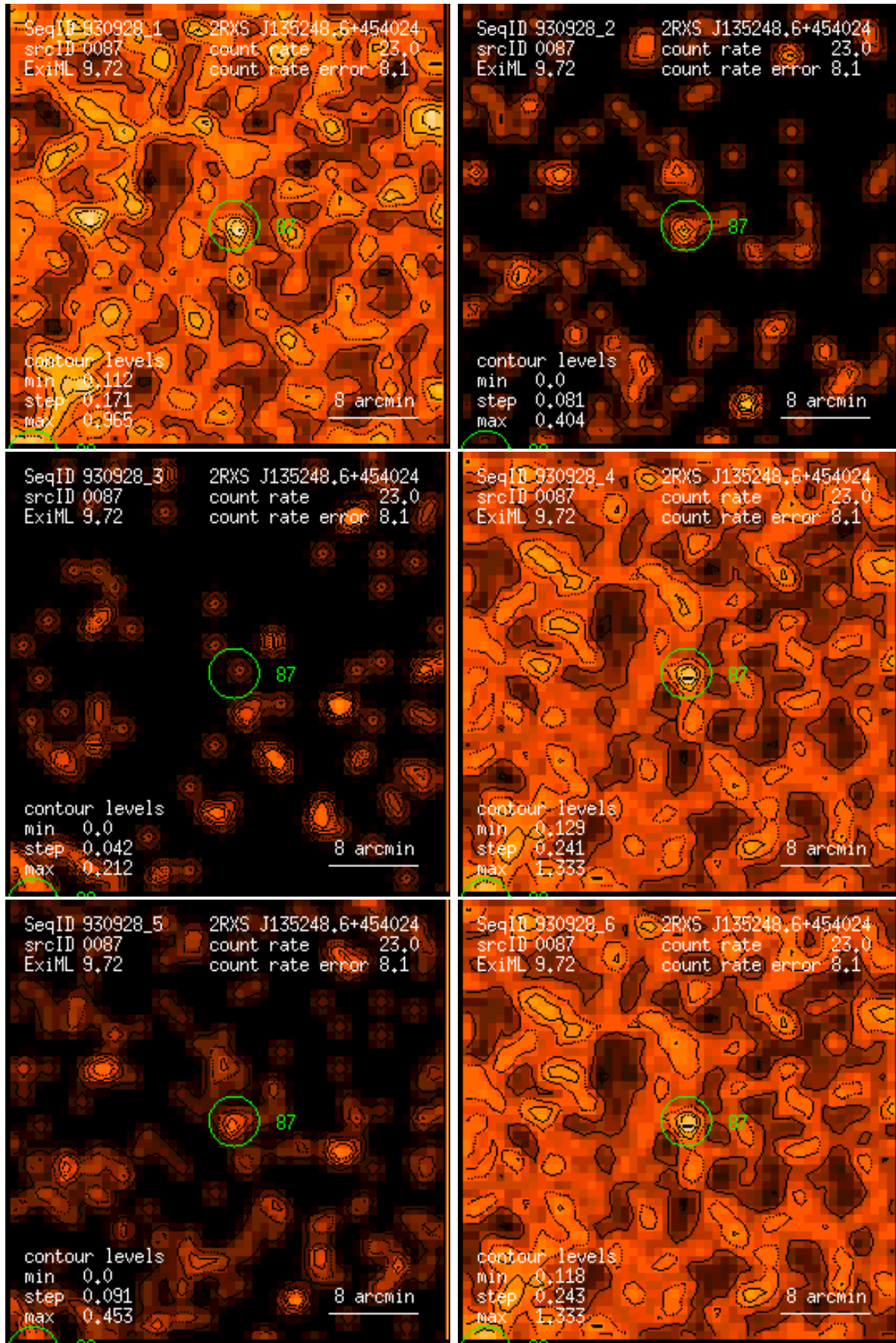
Figure 87: RASS 930928: detection 0087: band rate images, Gaussian filter: (1) PSPC channels 11 – 41, (2) 52 – 90, (3) 91 – 201, (4) 11 – 235, (5) 52 – 201, (6) 11 – 201. Broad band rates in counts/ks. Band rate contour levels in counts/ks/arcmin 2 .
