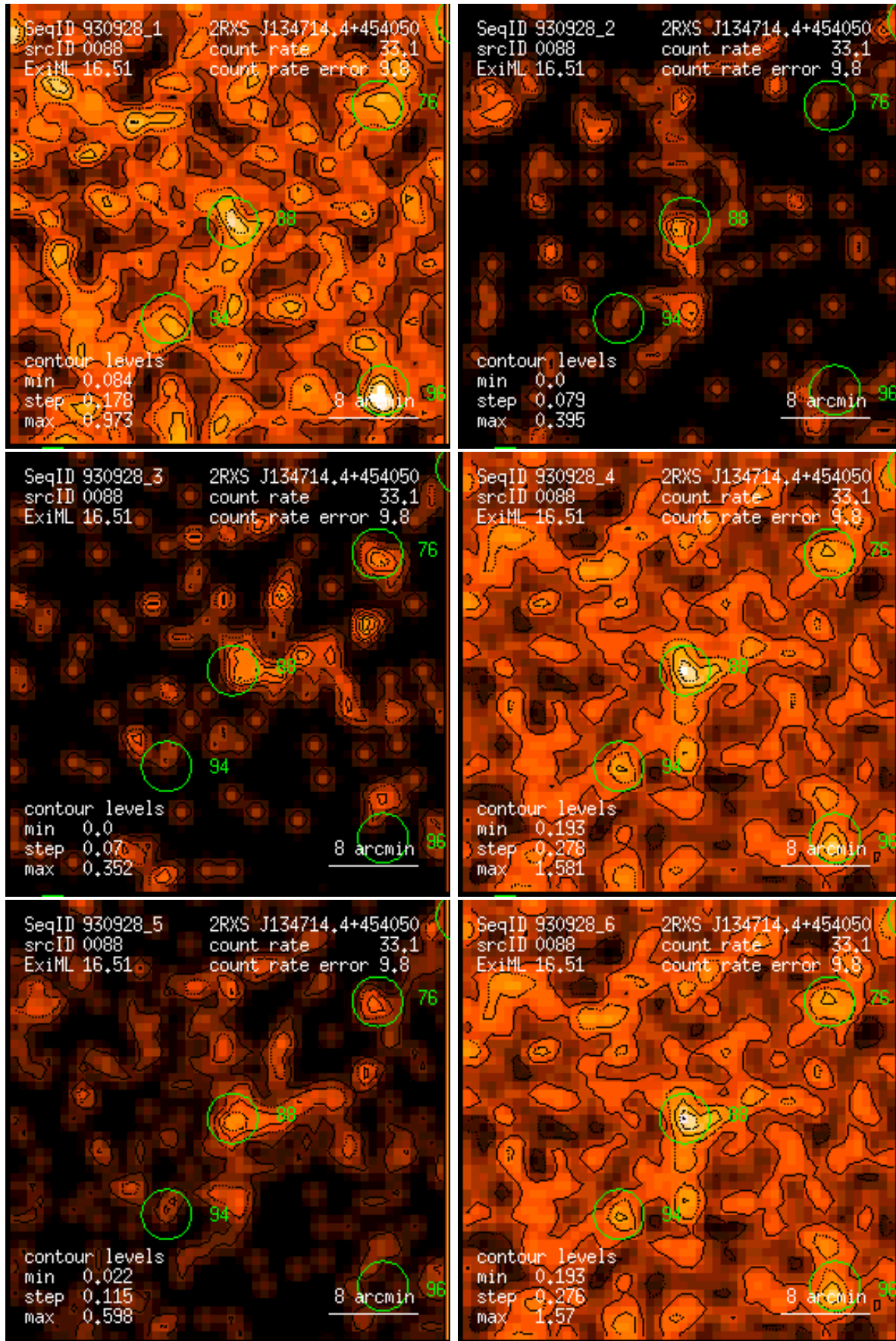
Figure 88: RASS 930928: detection 0088: band rate images, Gaussian filter: (1) PSPC channels 11 – 41, (2) 52 – 90, (3) 91 – 201, (4) 11 – 235, (5) 52 – 201, (6) 11 – 201. Broad band rates in counts/ks. Band rate contour levels in counts/ks/arcmin 2 .
