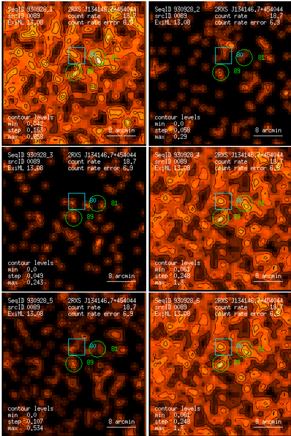
Figure 89: RASS 930928: detection 0089: band rate images, Gaussian filter: (1) PSPC channels 11 – 41, (2) 52 – 90, (3) 91 – 201, (4) 11 – 235, (5) 52 – 201, (6) 11 – 201. Broad band rates in counts/ks. Band rate contour levels in counts/ks/arcmin 2 .
