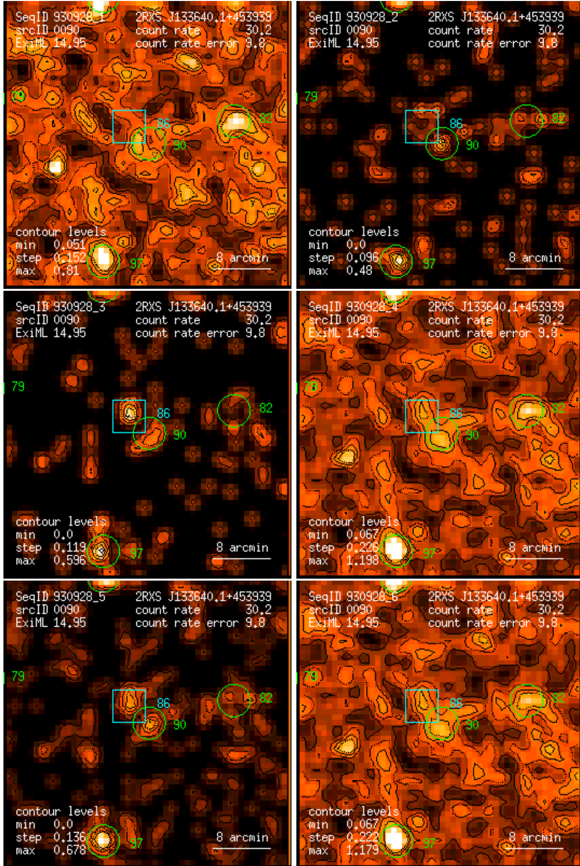
Figure 90: RASS 930928: detection 0090: band rate images, Gaussian filter: (1) PSPC channels 11 – 41, (2) 52 – 90, (3) 91 – 201, (4) 11 – 235, (5) 52 – 201, (6) 11 – 201. Broad band rates in counts/ks. Band rate contour levels in counts/ks/arcmin 2 .
