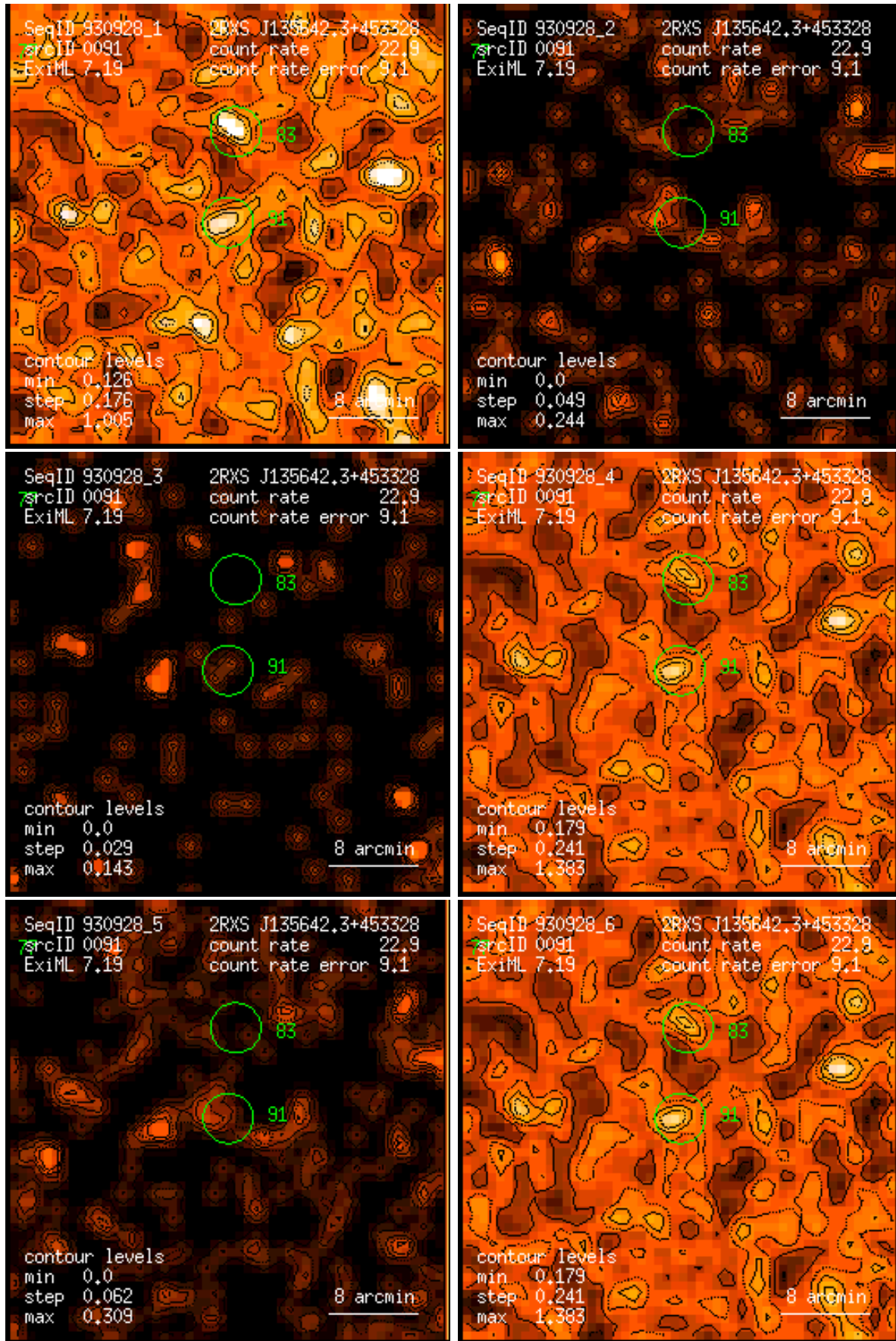
Figure 91: RASS 930928: detection 0091: band rate images, Gaussian filter: (1) PSPC channels 11 – 41, (2) 52 – 90, (3) 91 – 201, (4) 11 – 235, (5) 52 – 201, (6) 11 – 201. Broad band rates in counts/ks. Band rate contour levels in counts/ks/arcmin 2 .
