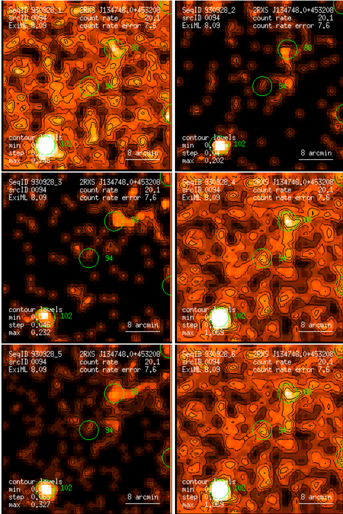
Figure 94: RASS 930928: detection 0094: band rate images, Gaussian filter: (1) PSPC channels 11 – 41, (2) 52 – 90, (3) 91 – 201, (4) 11 – 235, (5) 52 – 201, (6) 11 – 201. Broad band rates in counts/ks. Band rate contour levels in counts/ks/arcmin 2 .
