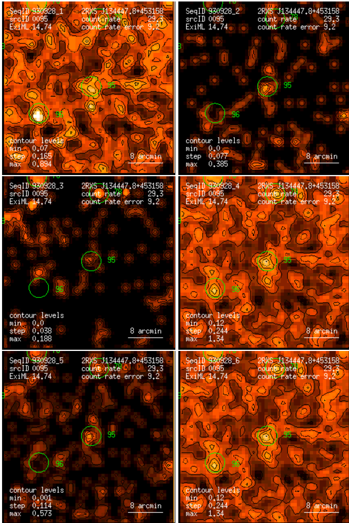
Figure 95: RASS 930928: detection 0095: band rate images, Gaussian filter: (1) PSPC channels 11 – 41, (2) 52 – 90, (3) 91 – 201, (4) 11 – 235, (5) 52 – 201, (6) 11 – 201. Broad band rates in counts/ks. Band rate contour levels in counts/ks/arcmin 2 .
