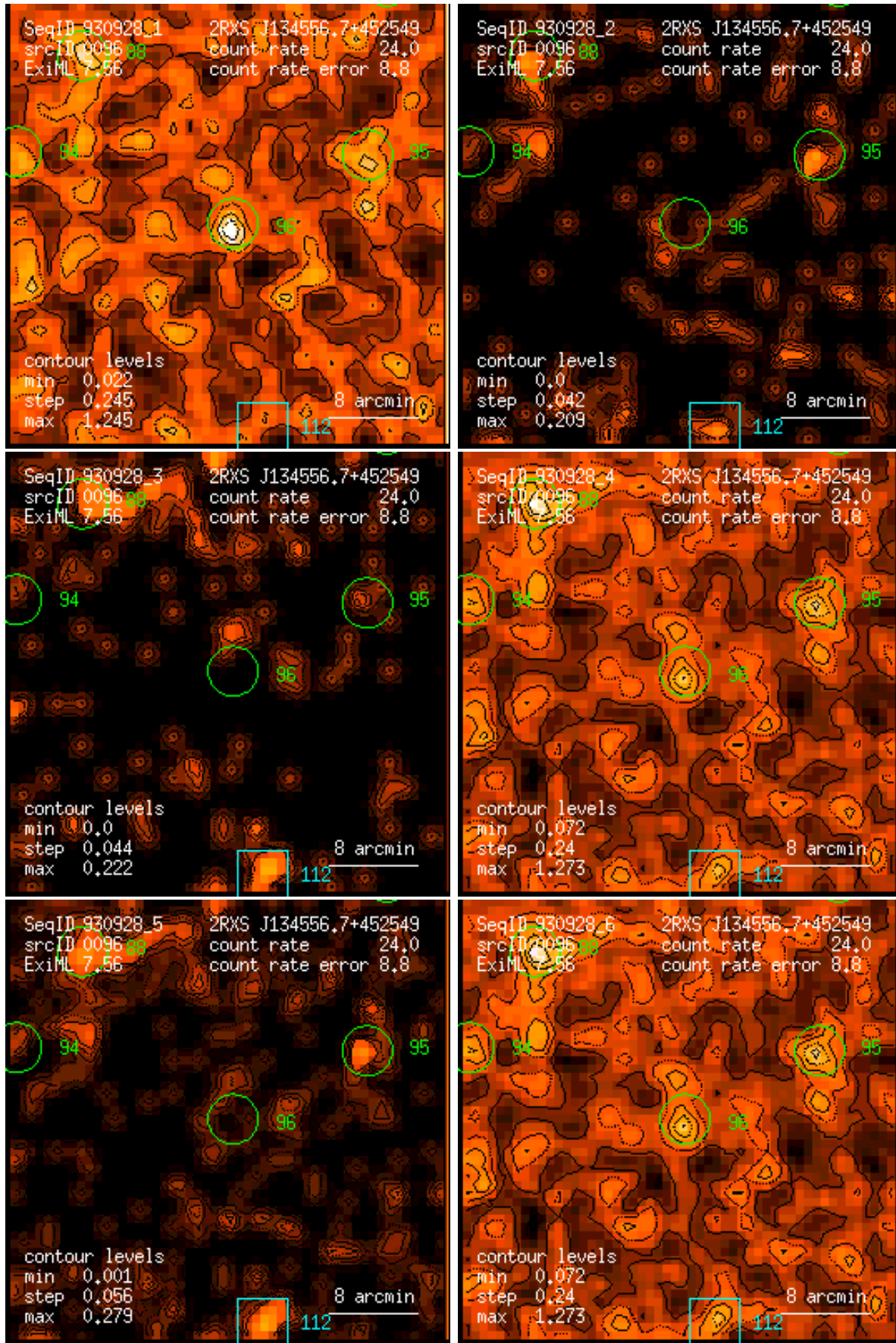
Figure 96: RASS 930928: detection 0096: band rate images, Gaussian filter: (1) PSPC channels 11 – 41, (2) 52 – 90, (3) 91 – 201, (4) 11 – 235, (5) 52 – 201, (6) 11 – 201. Broad band rates in counts/ks. Band rate contour levels in counts/ks/arcmin 2 .
