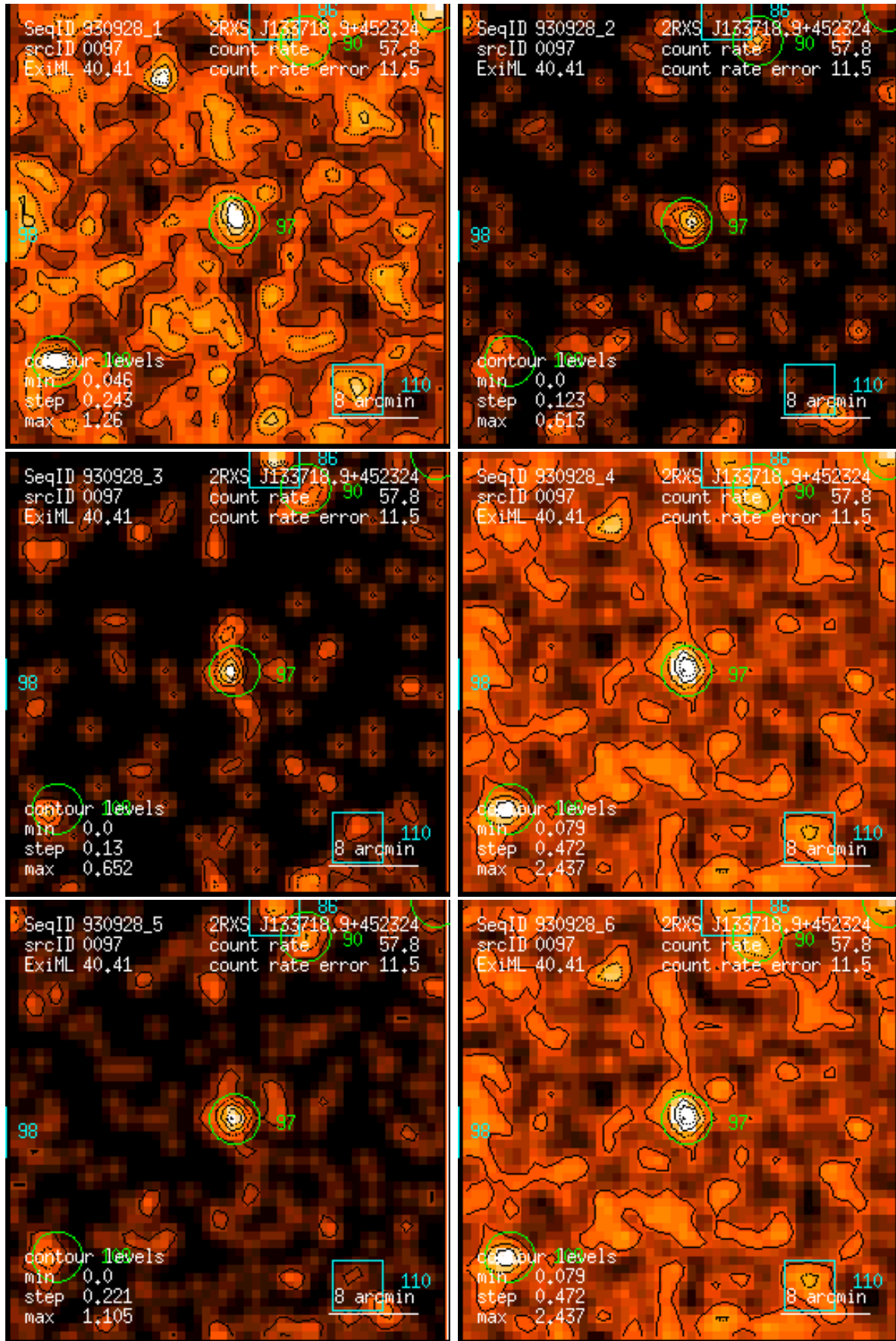
Figure 97: RASS 930928: detection 0097: band rate images, Gaussian filter: (1) PSPC channels 11 – 41, (2) 52 – 90, (3) 91 – 201, (4) 11 – 235, (5) 52 – 201, (6) 11 – 201. Broad band rates in counts/ks. Band rate contour levels in counts/ks/arcmin 2 .
