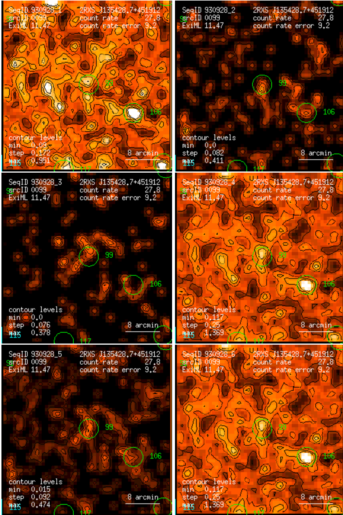
Figure 99: RASS 930928: detection 0099: band rate images, Gaussian filter: (1) PSPC channels 11 – 41, (2) 52 – 90, (3) 91 – 201, (4) 11 – 235, (5) 52 – 201, (6) 11 – 201. Broad band rates in counts/ks. Band rate contour levels in counts/ks/arcmin 2 .
