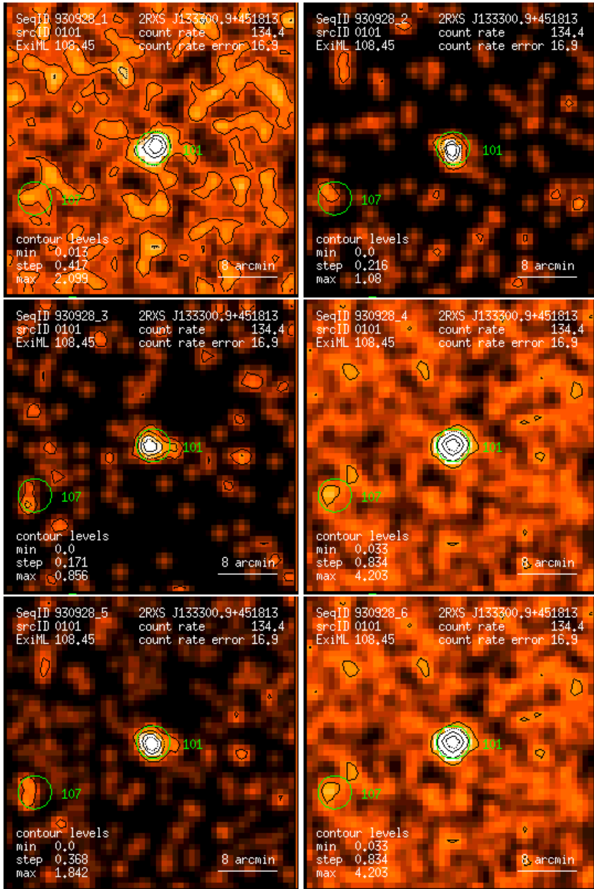
Figure 101: RASS 930928: detection 0101: band rate images, Gaussian filter: (1) PSPC channels 11 – 41, (2) 52 – 90, (3) 91 – 201, (4) 11 – 235, (5) 52 – 201, (6) 11 – 201. Broad band rates in counts/ks. Band rate contour levels in counts/ks/arcmin 2 .
