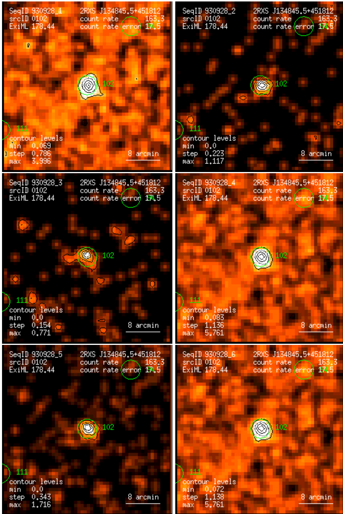
Figure 102: RASS 930928: detection 0102: band rate images, Gaussian filter: (1) PSPC channels 11 – 41, (2) 52 – 90, (3) 91 – 201, (4) 11 – 235, (5) 52 – 201, (6) 11 – 201. Broad band rates in counts/ks. Band rate contour levels in counts/ks/arcmin 2 .
