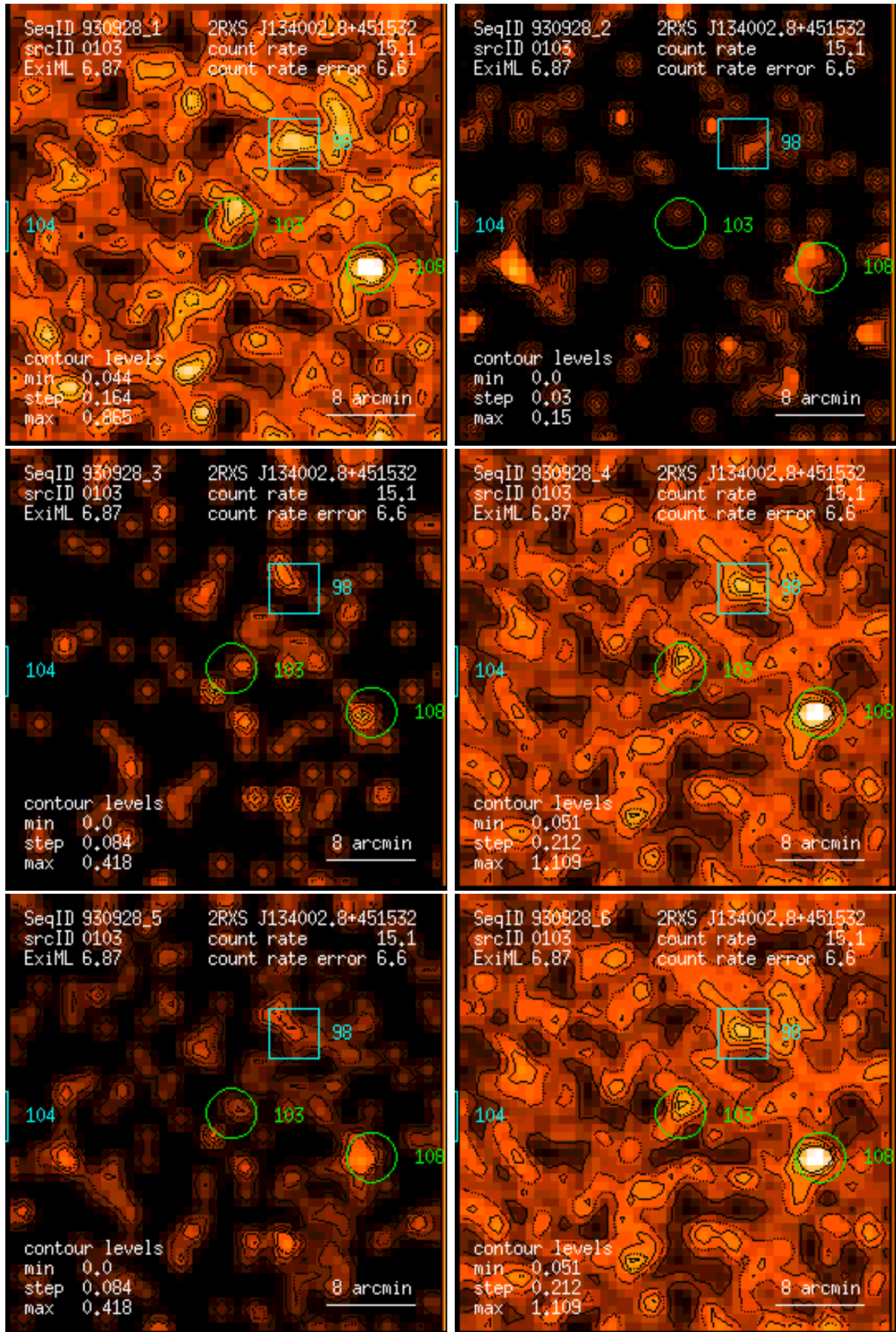
Figure 103: RASS 930928: detection 0103: band rate images, Gaussian filter: (1) PSPC channels 11 – 41, (2) 52 – 90, (3) 91 – 201, (4) 11 – 235, (5) 52 – 201, (6) 11 – 201. Broad band rates in counts/ks. Band rate contour levels in counts/ks/arcmin 2 .
