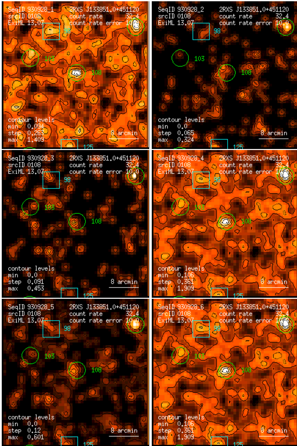
Figure 108: RASS 930928: detection 0108: band rate images, Gaussian filter: (1) PSPC channels 11 – 41, (2) 52 – 90, (3) 91 – 201, (4) 11 – 235, (5) 52 – 201, (6) 11 – 201. Broad band rates in counts/ks. Band rate contour levels in counts/ks/arcmin 2 .
