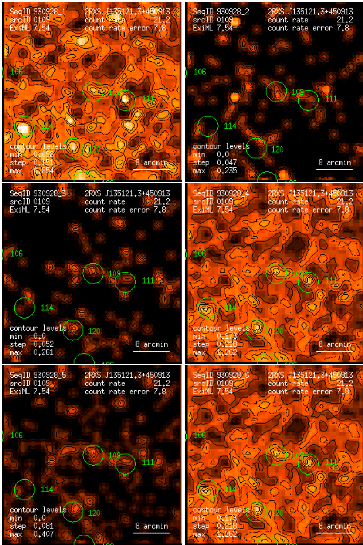
Figure 109: RASS 930928: detection 0109: band rate images, Gaussian filter: (1) PSPC channels 11 – 41, (2) 52 – 90, (3) 91 – 201, (4) 11 – 235, (5) 52 – 201, (6) 11 – 201. Broad band rates in counts/ks. Band rate contour levels in counts/ks/arcmin 2 .
