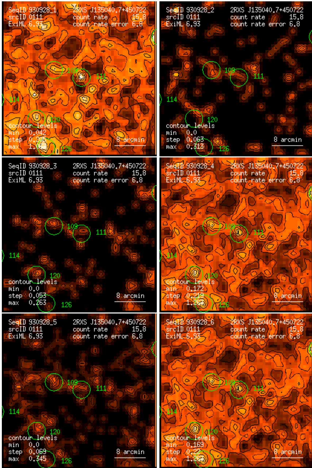
Figure 111: RASS 930928: detection 0111: band rate images, Gaussian filter: (1) PSPC channels 11 – 41, (2) 52 – 90, (3) 91 – 201, (4) 11 – 235, (5) 52 – 201, (6) 11 – 201. Broad band rates in counts/ks. Band rate contour levels in counts/ks/arcmin 2 .
