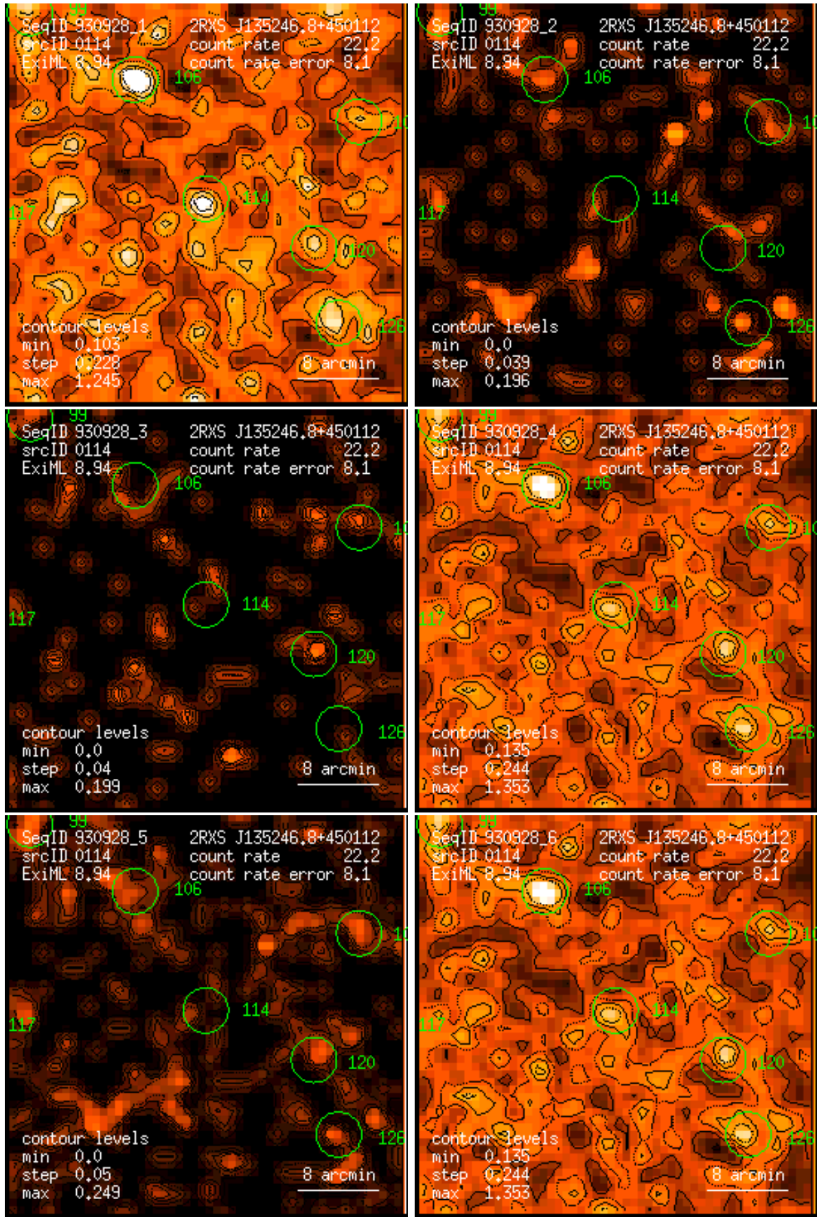
Figure 114: RASS 930928: detection 0114: band rate images, Gaussian filter: (1) PSPC channels 11 – 41, (2) 52 – 90, (3) 91 – 201, (4) 11 – 235, (5) 52 – 201, (6) 11 – 201. Broad band rates in counts/ks. Band rate contour levels in counts/ks/arcmin 2 .
