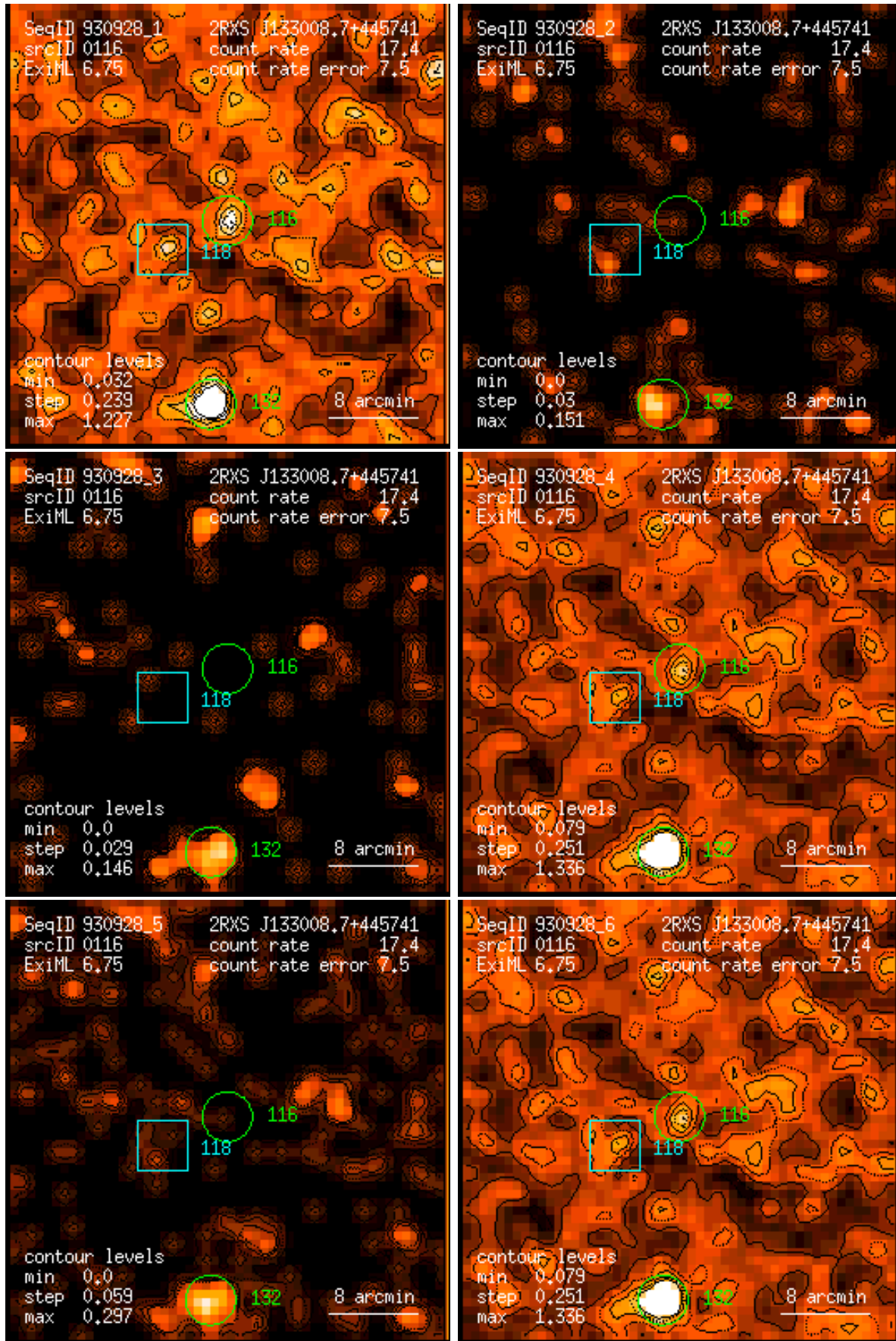
Figure 116: RASS 930928: detection 0116: band rate images, Gaussian filter: (1) PSPC channels 11 – 41, (2) 52 – 90, (3) 91 – 201, (4) 11 – 235, (5) 52 – 201, (6) 11 – 201. Broad band rates in counts/ks. Band rate contour levels in counts/ks/arcmin 2 .
