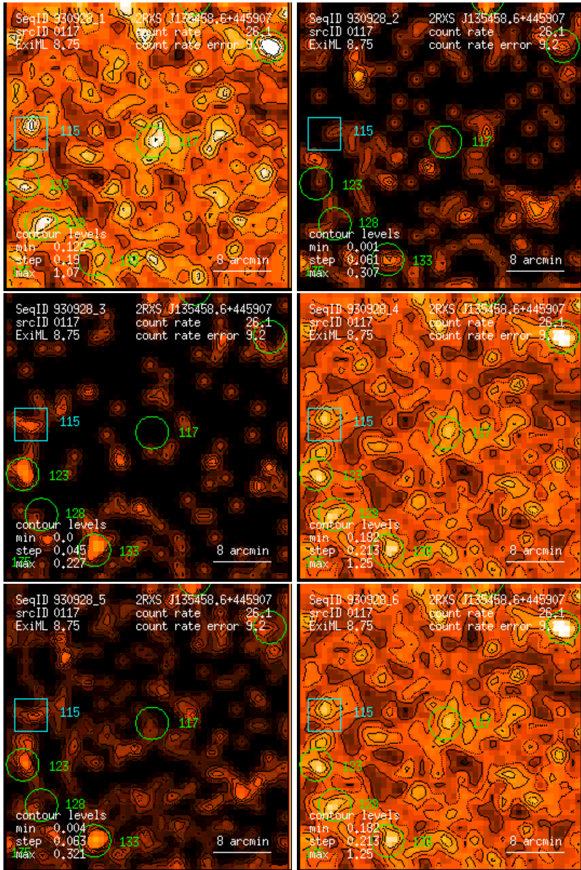
Figure 117: RASS 930928: detection 0117: band rate images, Gaussian filter: (1) PSPC channels 11 – 41, (2) 52 – 90, (3) 91 – 201, (4) 11 – 235, (5) 52 – 201, (6) 11 – 201. Broad band rates in counts/ks. Band rate contour levels in counts/ks/arcmin 2 .
