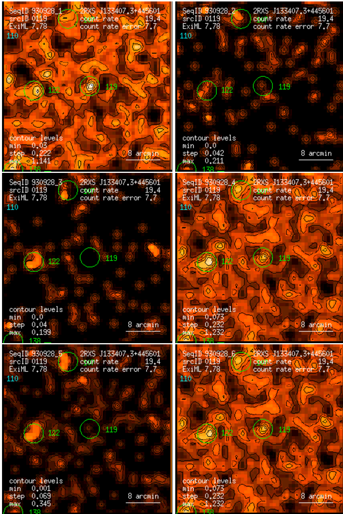
Figure 119: RASS 930928: detection 0119: band rate images, Gaussian filter: (1) PSPC channels 11 – 41, (2) 52 – 90, (3) 91 – 201, (4) 11 – 235, (5) 52 – 201, (6) 11 – 201. Broad band rates in counts/ks. Band rate contour levels in counts/ks/arcmin 2 .
