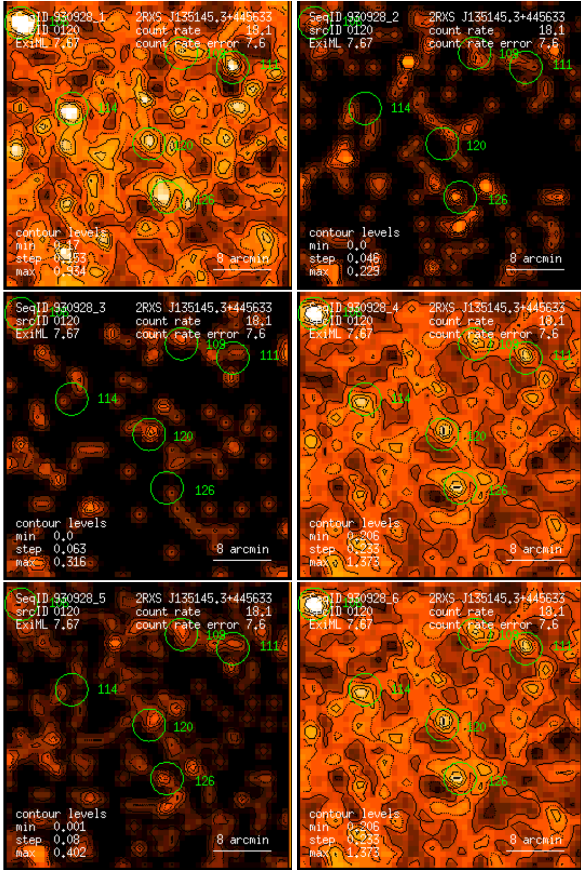
Figure 120: RASS 930928: detection 0120: band rate images, Gaussian filter: (1) PSPC channels 11 – 41, (2) 52 – 90, (3) 91 – 201, (4) 11 – 235, (5) 52 – 201, (6) 11 – 201. Broad band rates in counts/ks. Band rate contour levels in counts/ks/arcmin 2 .
