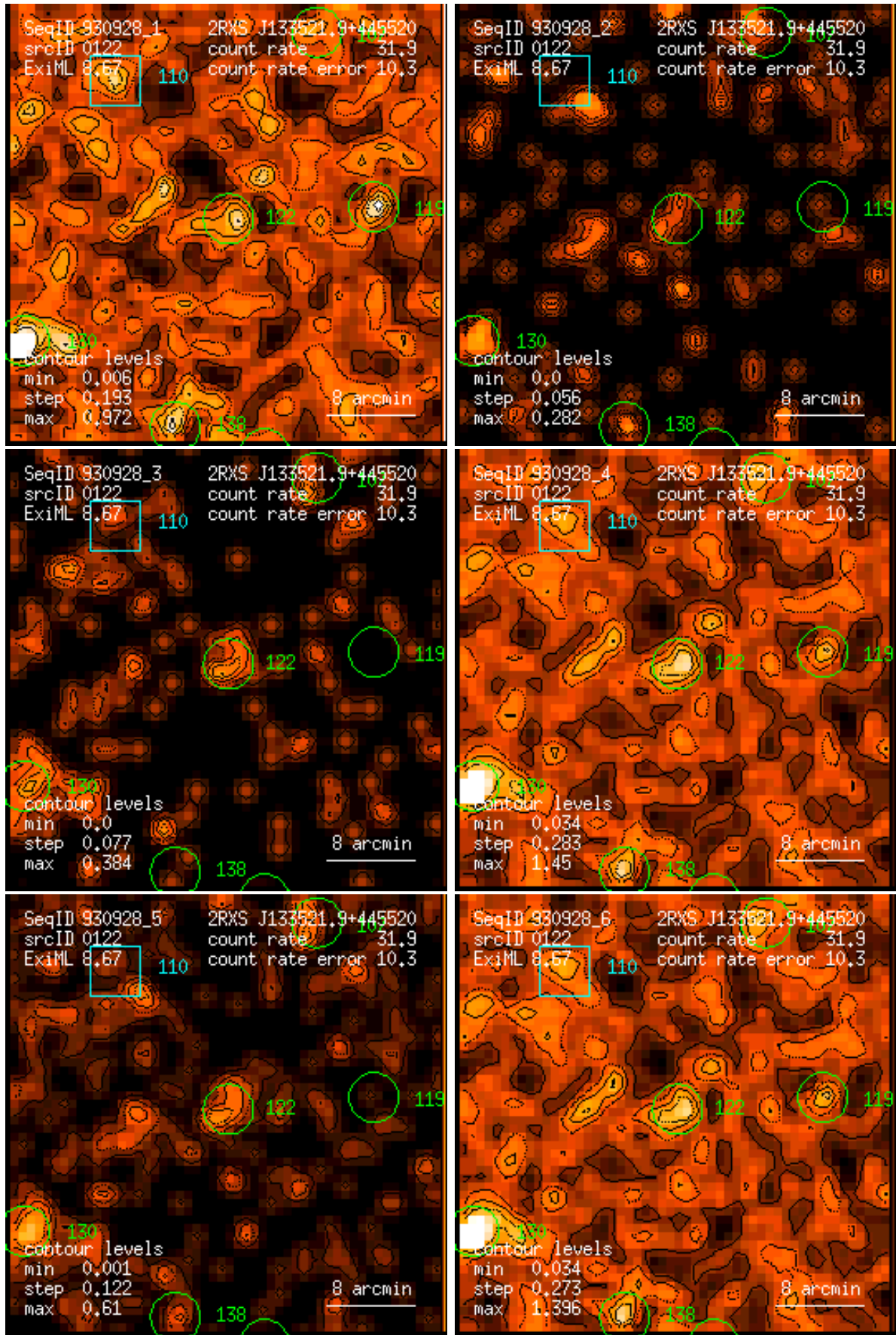
Figure 122: RASS 930928: detection 0122: band rate images, Gaussian filter: (1) PSPC channels 11 – 41, (2) 52 – 90, (3) 91 – 201, (4) 11 – 235, (5) 52 – 201, (6) 11 – 201. Broad band rates in counts/ks. Band rate contour levels in counts/ks/arcmin 2 .
