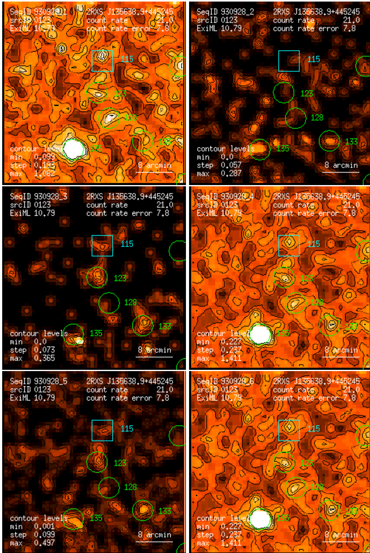
Figure 123: RASS 930928: detection 0123: band rate images, Gaussian filter: (1) PSPC channels 11 – 41, (2) 52 – 90, (3) 91 – 201, (4) 11 – 235, (5) 52 – 201, (6) 11 – 201. Broad band rates in counts/ks. Band rate contour levels in counts/ks/arcmin 2 .
