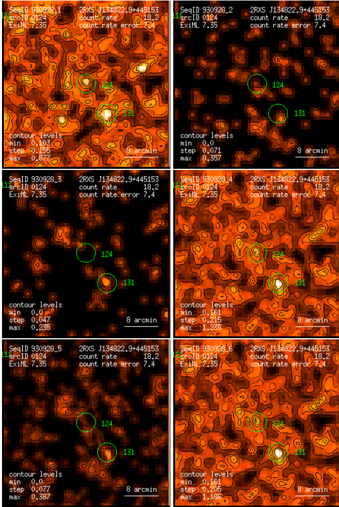
Figure 124: RASS 930928: detection 0124: band rate images, Gaussian filter: (1) PSPC channels 11 – 41, (2) 52 – 90, (3) 91 – 201, (4) 11 – 235, (5) 52 – 201, (6) 11 – 201. Broad band rates in counts/ks. Band rate contour levels in counts/ks/arcmin 2 .
