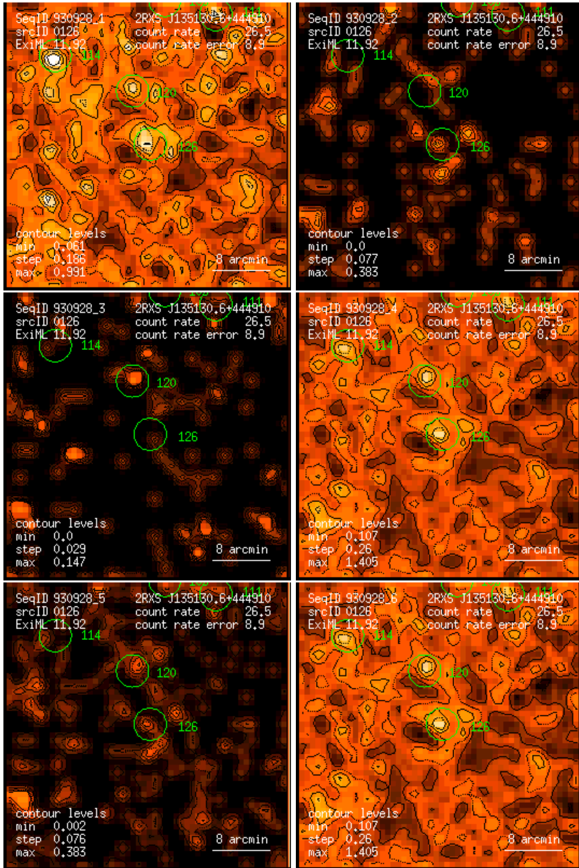
Figure 126: RASS 930928: detection 0126: band rate images, Gaussian filter: (1) PSPC channels 11 – 41, (2) 52 – 90, (3) 91 – 201, (4) 11 – 235, (5) 52 – 201, (6) 11 – 201. Broad band rates in counts/ks. Band rate contour levels in counts/ks/arcmin 2 .
