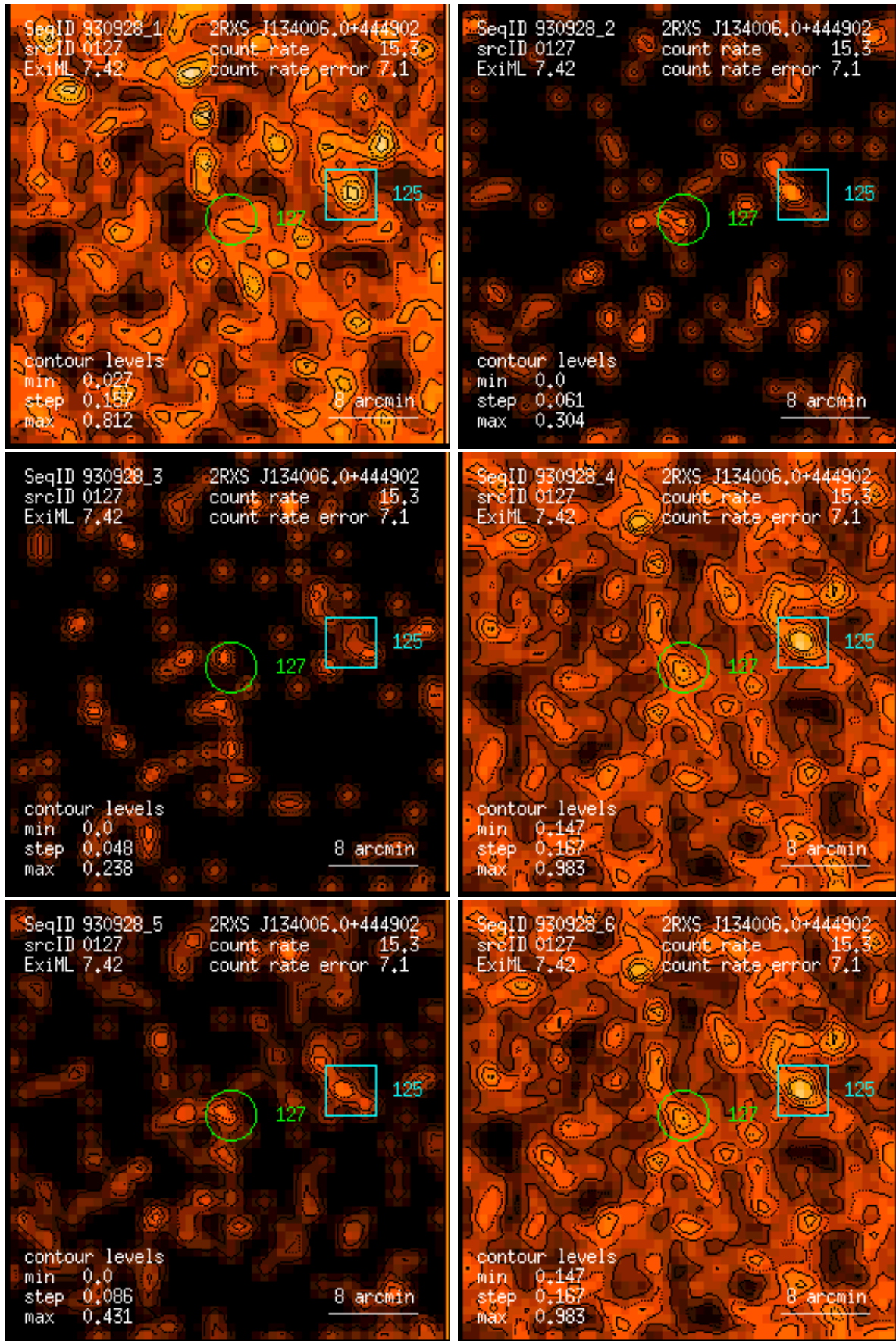
Figure 127: RASS 930928: detection 0127: band rate images, Gaussian filter: (1) PSPC channels 11 – 41, (2) 52 – 90, (3) 91 – 201, (4) 11 – 235, (5) 52 – 201, (6) 11 – 201. Broad band rates in counts/ks. Band rate contour levels in counts/ks/arcmin 2 .
