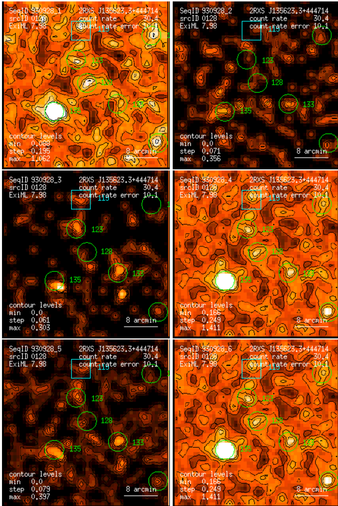
Figure 128: RASS 930928: detection 0128: band rate images, Gaussian filter: (1) PSPC channels 11 – 41, (2) 52 – 90, (3) 91 – 201, (4) 11 – 235, (5) 52 – 201, (6) 11 – 201. Broad band rates in counts/ks. Band rate contour levels in counts/ks/arcmin 2 .
