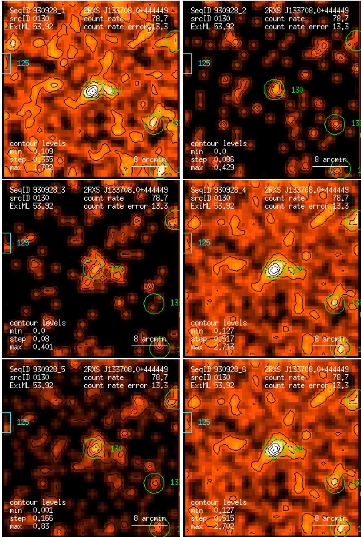
Figure 130: RASS 930928: detection 0130: band rate images, Gaussian filter: (1) PSPC channels 11 – 41, (2) 52 – 90, (3) 91 – 201, (4) 11 – 235, (5) 52 – 201, (6) 11 – 201. Broad band rates in counts/ks. Band rate contour levels in counts/ks/arcmin 2 .
