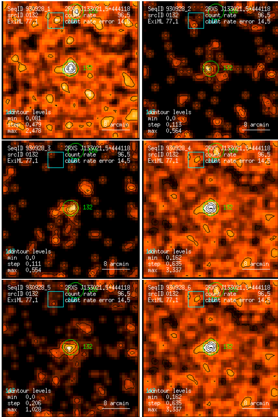
Figure 132: RASS 930928: detection 0132: band rate images, Gaussian filter: (1) PSPC channels 11 – 41, (2) 52 – 90, (3) 91 – 201, (4) 11 – 235, (5) 52 – 201, (6) 11 – 201. Broad band rates in counts/ks. Band rate contour levels in counts/ks/arcmin 2 .
