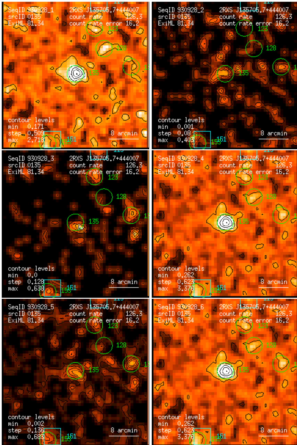
Figure 135: RASS 930928: detection 0135: band rate images, Gaussian filter: (1) PSPC channels 11 – 41, (2) 52 – 90, (3) 91 – 201, (4) 11 – 235, (5) 52 – 201, (6) 11 – 201. Broad band rates in counts/ks. Band rate contour levels in counts/ks/arcmin 2 .
