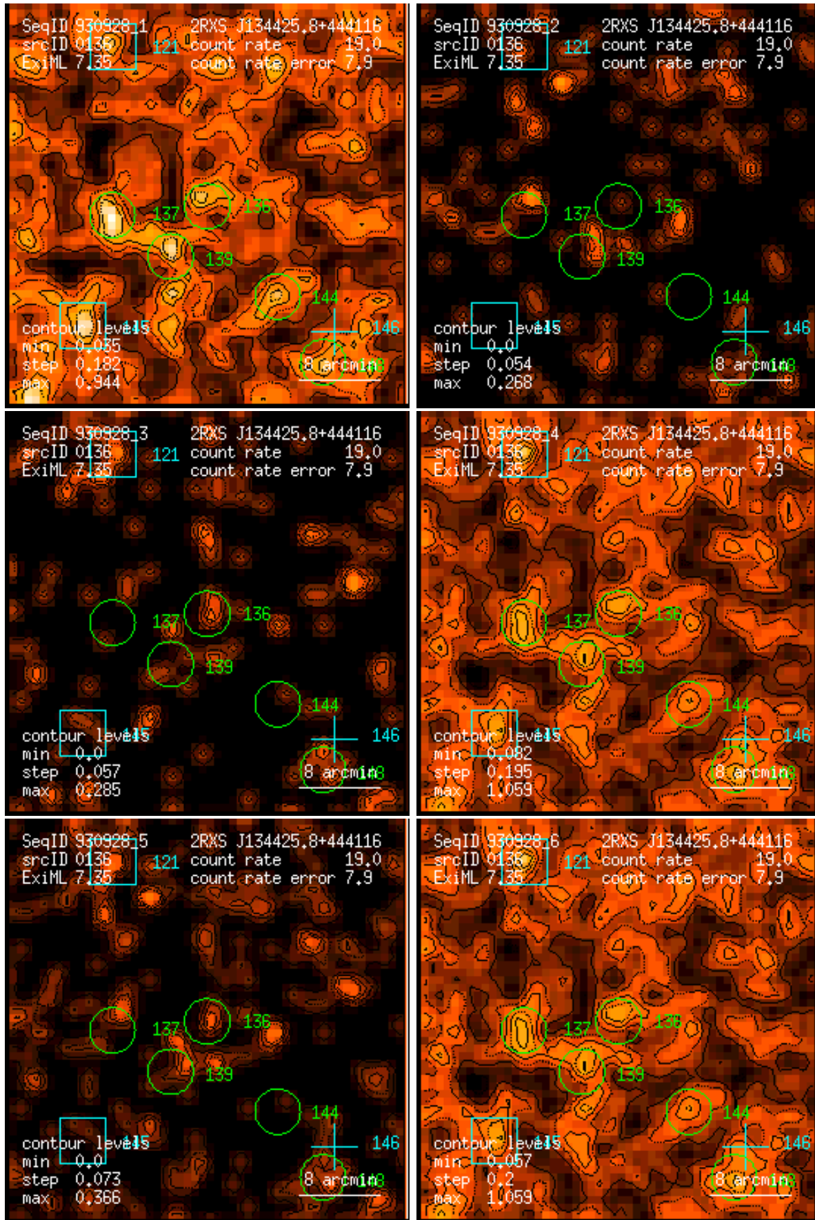
Figure 136: RASS 930928: detection 0136: band rate images, Gaussian filter: (1) PSPC channels 11 – 41, (2) 52 – 90, (3) 91 – 201, (4) 11 – 235, (5) 52 – 201, (6) 11 – 201. Broad band rates in counts/ks. Band rate contour levels in counts/ks/arcmin 2 .
