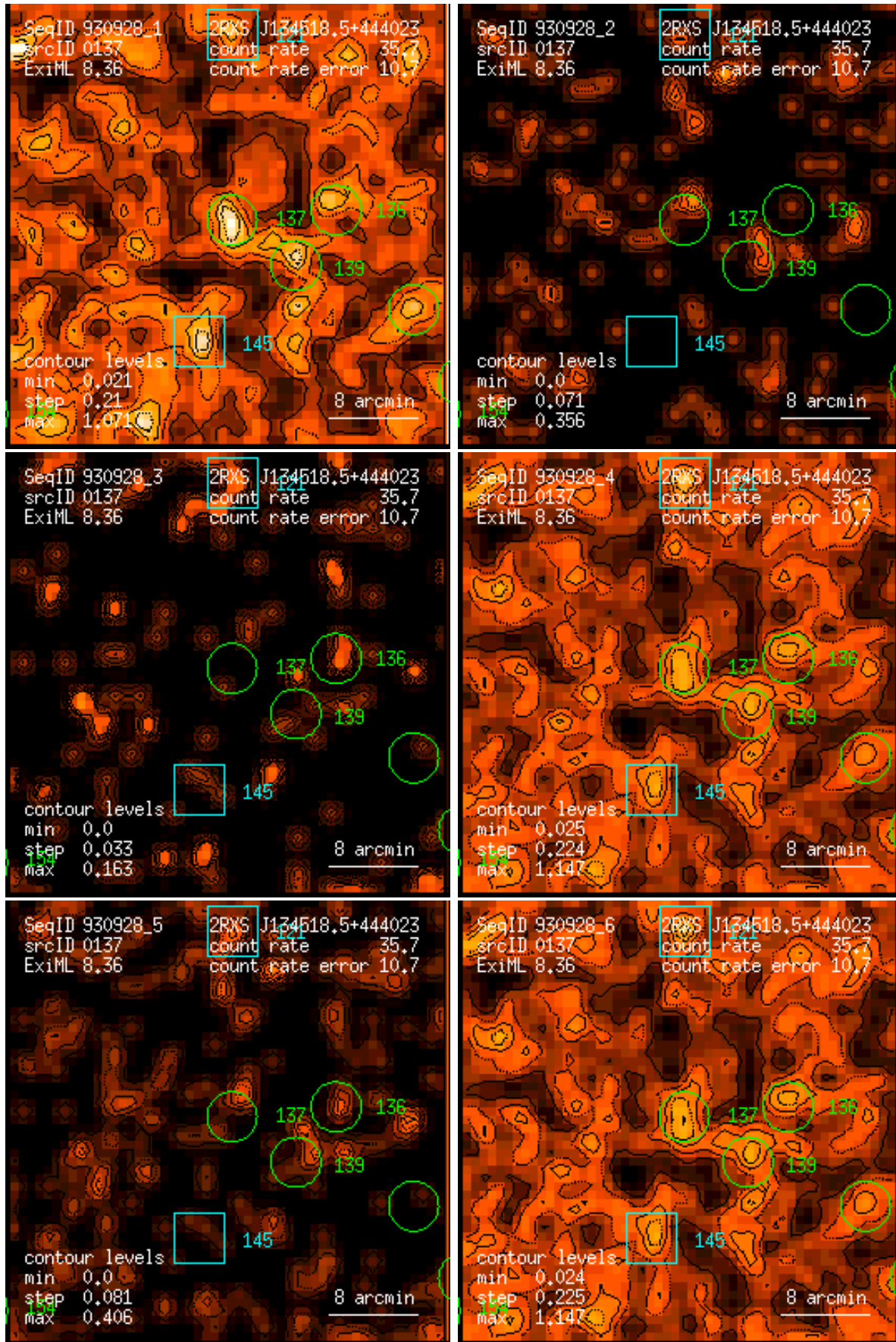
Figure 137: RASS 930928: detection 0137: band rate images, Gaussian filter: (1) PSPC channels 11 – 41, (2) 52 – 90, (3) 91 – 201, (4) 11 – 235, (5) 52 – 201, (6) 11 – 201. Broad band rates in counts/ks. Band rate contour levels in counts/ks/arcmin 2 .
