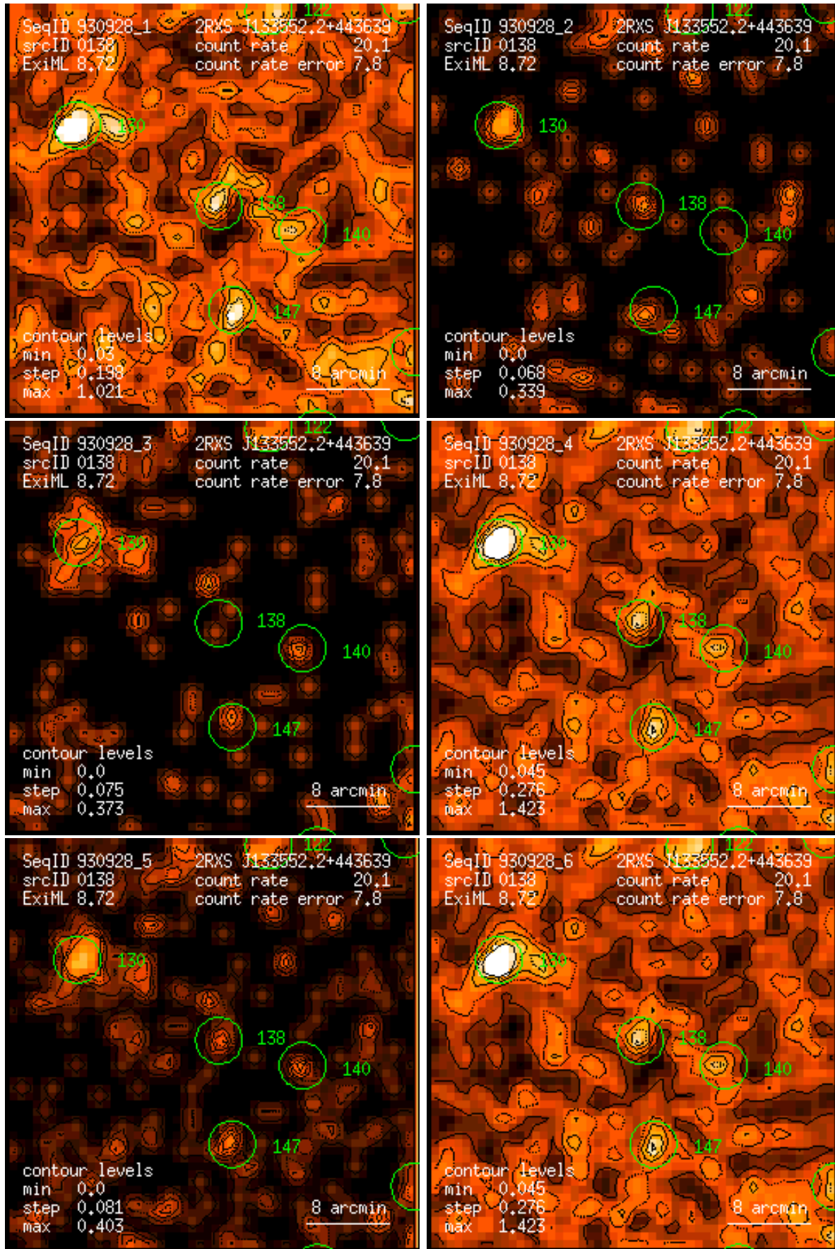
Figure 138: RASS 930928: detection 0138: band rate images, Gaussian filter: (1) PSPC channels 11 – 41, (2) 52 – 90, (3) 91 – 201, (4) 11 – 235, (5) 52 – 201, (6) 11 – 201. Broad band rates in counts/ks. Band rate contour levels in counts/ks/arcmin 2 .
