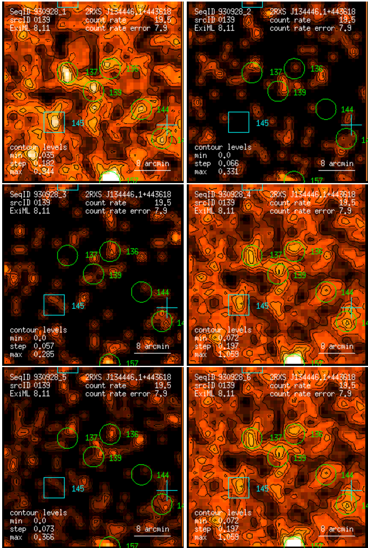
Figure 139: RASS 930928: detection 0139: band rate images, Gaussian filter: (1) PSPC channels 11 – 41, (2) 52 – 90, (3) 91 – 201, (4) 11 – 235, (5) 52 – 201, (6) 11 – 201. Broad band rates in counts/ks. Band rate contour levels in counts/ks/arcmin 2 .
