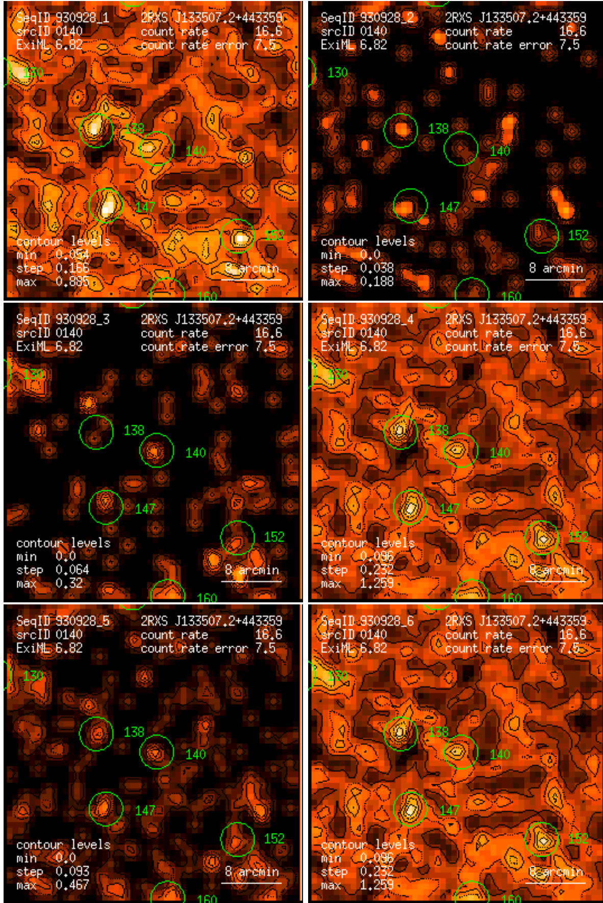
Figure 140: RASS 930928: detection 0140: band rate images, Gaussian filter: (1) PSPC channels 11 – 41, (2) 52 – 90, (3) 91 – 201, (4) 11 – 235, (5) 52 – 201, (6) 11 – 201. Broad band rates in counts/ks. Band rate contour levels in counts/ks/arcmin 2 .
