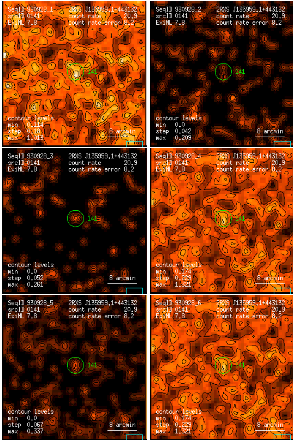
Figure 141: RASS 930928: detection 0141: band rate images, Gaussian filter: (1) PSPC channels 11 – 41, (2) 52 – 90, (3) 91 – 201, (4) 11 – 235, (5) 52 – 201, (6) 11 – 201. Broad band rates in counts/ks. Band rate contour levels in counts/ks/arcmin 2 .
