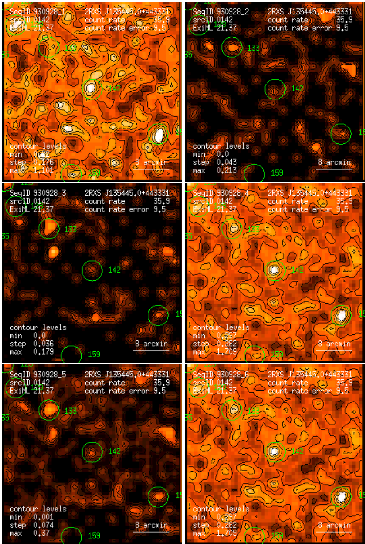
Figure 142: RASS 930928: detection 0142: band rate images, Gaussian filter: (1) PSPC channels 11 – 41, (2) 52 – 90, (3) 91 – 201, (4) 11 – 235, (5) 52 – 201, (6) 11 – 201. Broad band rates in counts/ks. Band rate contour levels in counts/ks/arcmin 2 .
