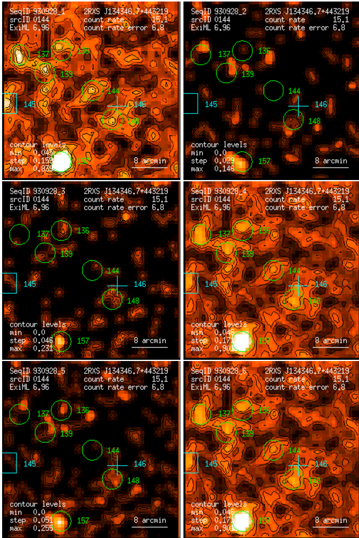
Figure 144: RASS 930928: detection 0144: band rate images, Gaussian filter: (1) PSPC channels 11 – 41, (2) 52 – 90, (3) 91 – 201, (4) 11 – 235, (5) 52 – 201, (6) 11 – 201. Broad band rates in counts/ks. Band rate contour levels in counts/ks/arcmin 2 .
