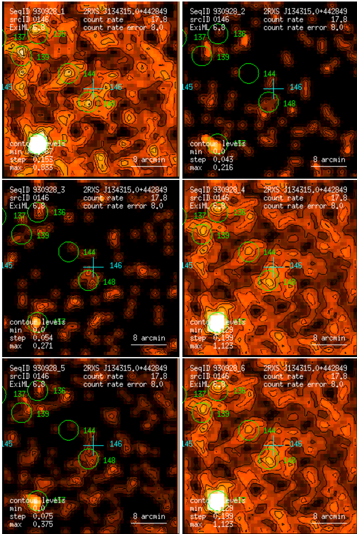
Figure 146: RASS 930928: detection 0146: band rate images, Gaussian filter: (1) PSPC channels 11 – 41, (2) 52 – 90, (3) 91 – 201, (4) 11 – 235, (5) 52 – 201, (6) 11 – 201. Broad band rates in counts/ks. Band rate contour levels in counts/ks/arcmin 2 .
