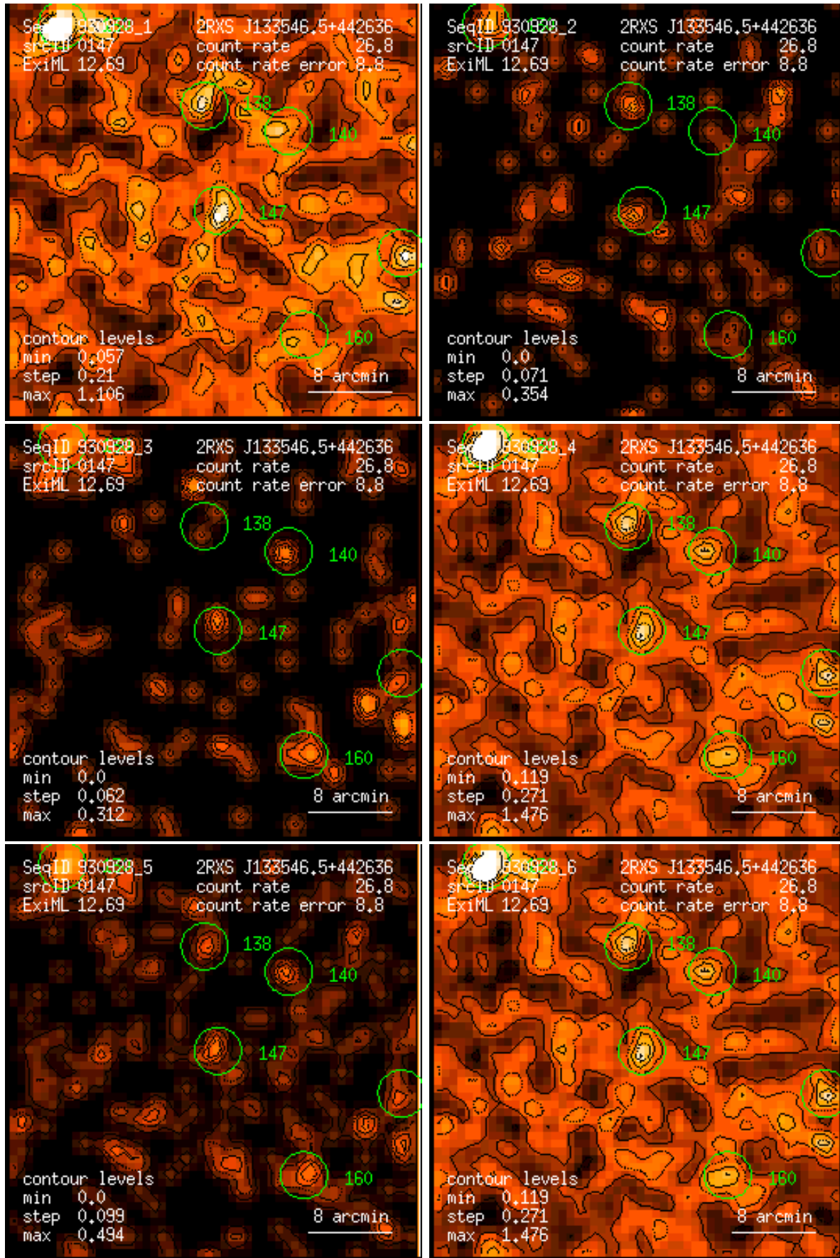
Figure 147: RASS 930928: detection 0147: band rate images, Gaussian filter: (1) PSPC channels 11 – 41, (2) 52 – 90, (3) 91 – 201, (4) 11 – 235, (5) 52 – 201, (6) 11 – 201. Broad band rates in counts/ks. Band rate contour levels in counts/ks/arcmin 2 .
