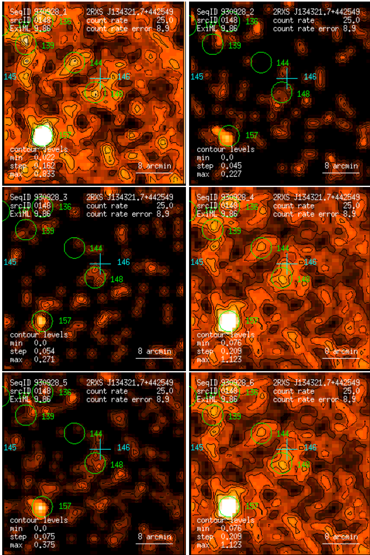
Figure 148: RASS 930928: detection 0148: band rate images, Gaussian filter: (1) PSPC channels 11 – 41, (2) 52 – 90, (3) 91 – 201, (4) 11 – 235, (5) 52 – 201, (6) 11 – 201. Broad band rates in counts/ks. Band rate contour levels in counts/ks/arcmin 2 .
