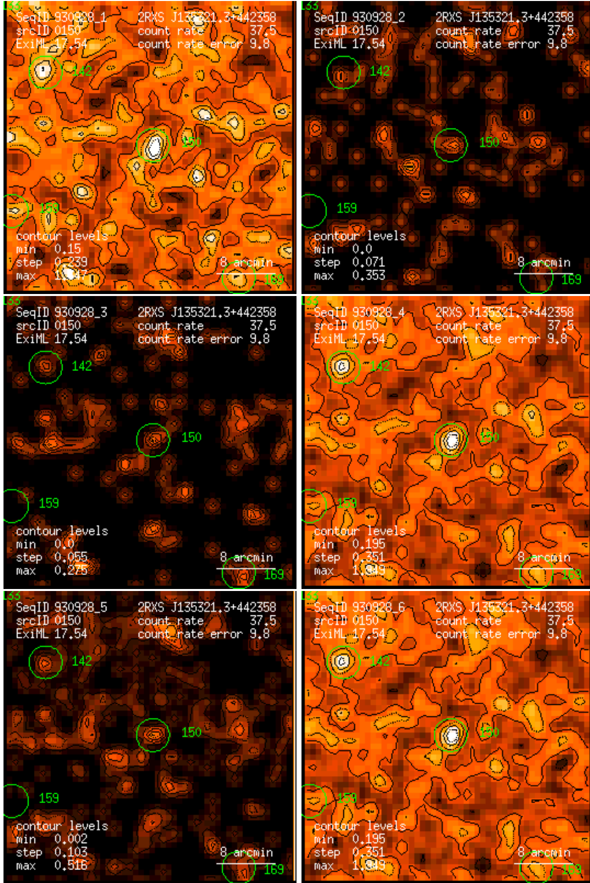
Figure 150: RASS 930928: detection 0150: band rate images, Gaussian filter: (1) PSPC channels 11 – 41, (2) 52 – 90, (3) 91 – 201, (4) 11 – 235, (5) 52 – 201, (6) 11 – 201. Broad band rates in counts/ks. Band rate contour levels in counts/ks/arcmin 2 .
