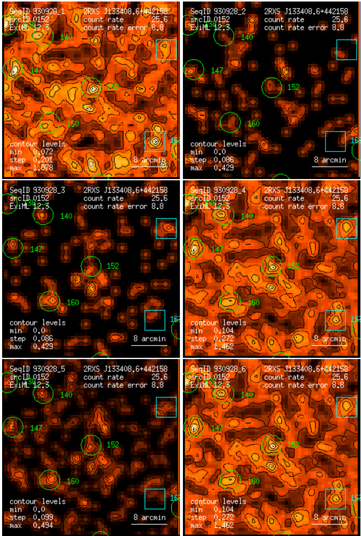
Figure 152: RASS 930928: detection 0152: band rate images, Gaussian filter: (1) PSPC channels 11 – 41, (2) 52 – 90, (3) 91 – 201, (4) 11 – 235, (5) 52 – 201, (6) 11 – 201. Broad band rates in counts/ks. Band rate contour levels in counts/ks/arcmin 2 .
