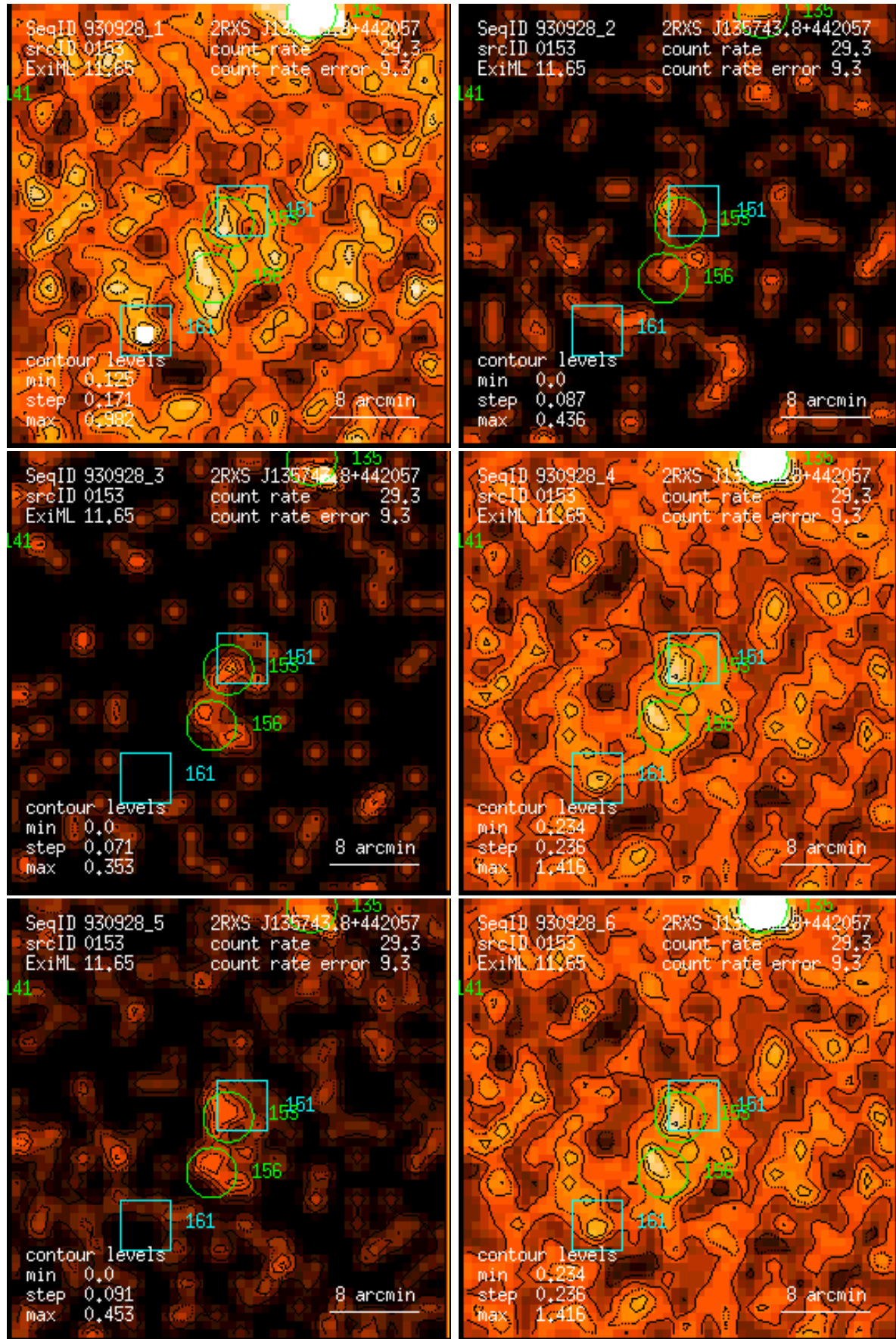
Figure 153: RASS 930928: detection 0153: band rate images, Gaussian filter: (1) PSPC channels 11 – 41, (2) 52 – 90, (3) 91 – 201, (4) 11 – 235, (5) 52 – 201, (6) 11 – 201. Broad band rates in counts/ks. Band rate contour levels in counts/ks/arcmin 2 .
