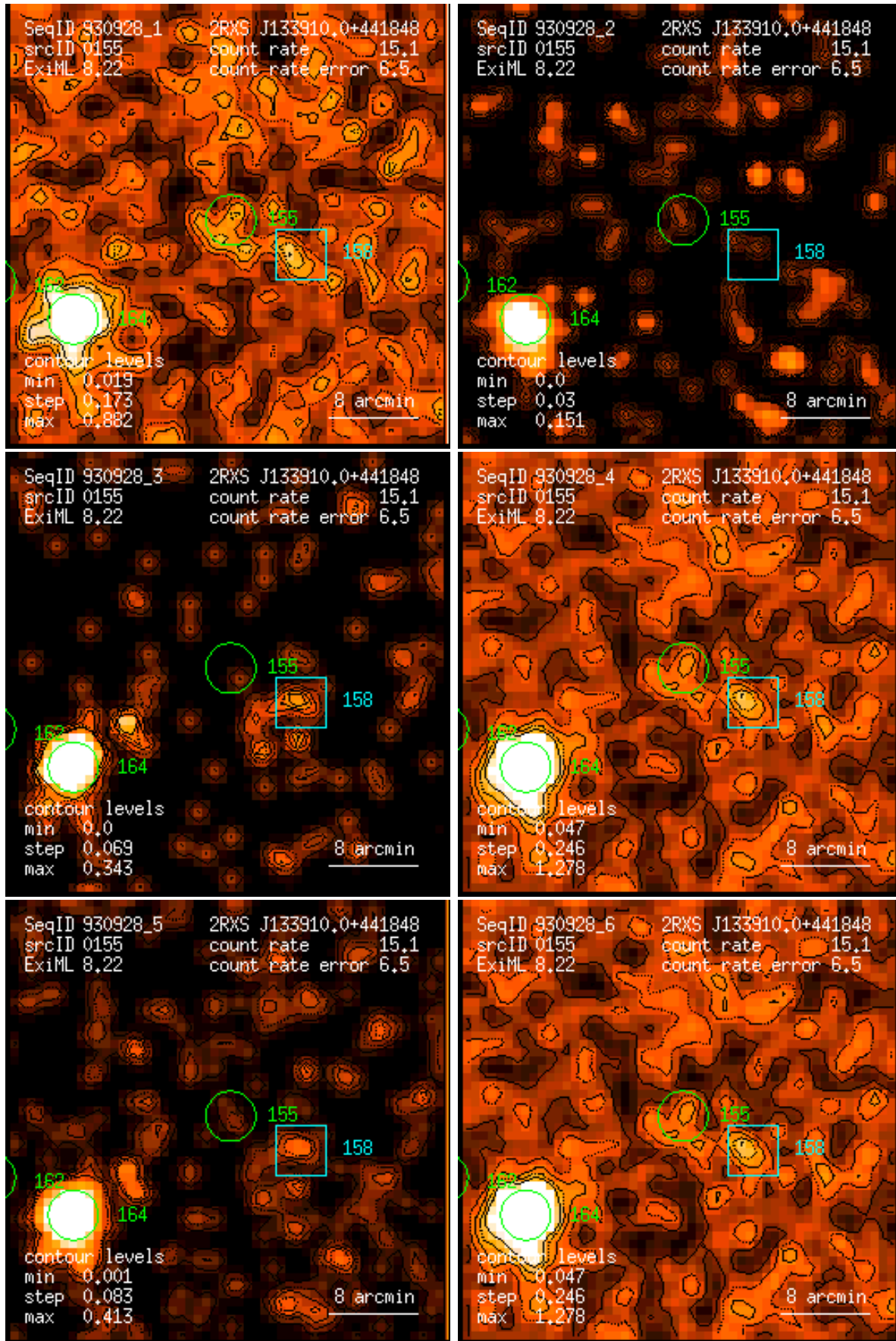
Figure 155: RASS 930928: detection 0155: band rate images, Gaussian filter: (1) PSPC channels 11 – 41, (2) 52 – 90, (3) 91 – 201, (4) 11 – 235, (5) 52 – 201, (6) 11 – 201. Broad band rates in counts/ks. Band rate contour levels in counts/ks/arcmin 2 .
