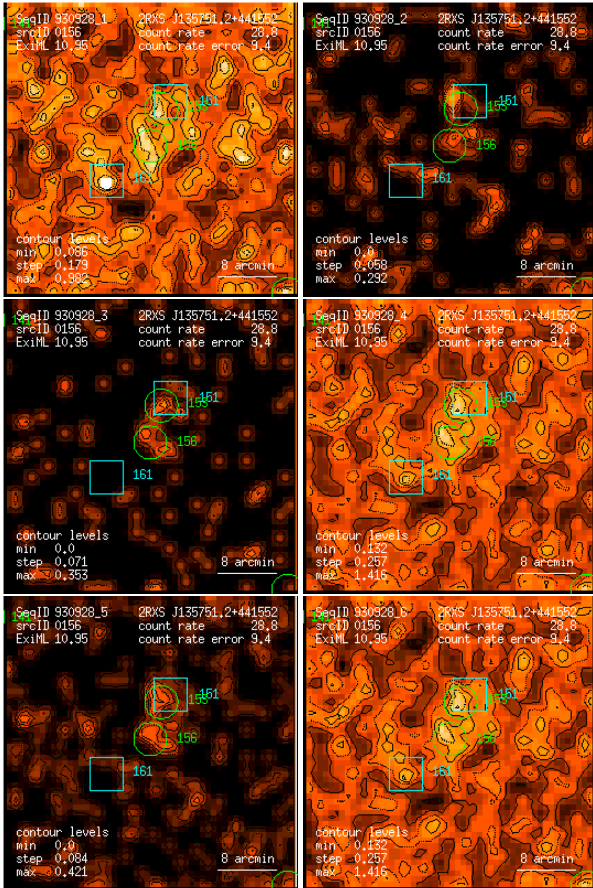
Figure 156: RASS 930928: detection 0156: band rate images, Gaussian filter: (1) PSPC channels 11 – 41, (2) 52 – 90, (3) 91 – 201, (4) 11 – 235, (5) 52 – 201, (6) 11 – 201. Broad band rates in counts/ks. Band rate contour levels in counts/ks/arcmin 2 .
