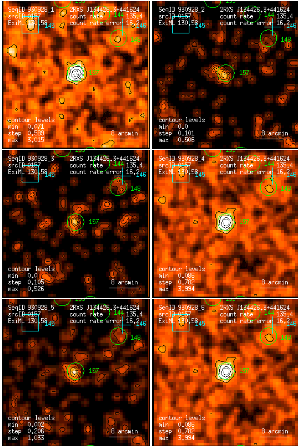
Figure 157: RASS 930928: detection 0157: band rate images, Gaussian filter: (1) PSPC channels 11 – 41, (2) 52 – 90, (3) 91 – 201, (4) 11 – 235, (5) 52 – 201, (6) 11 – 201. Broad band rates in counts/ks. Band rate contour levels in counts/ks/arcmin 2 .
